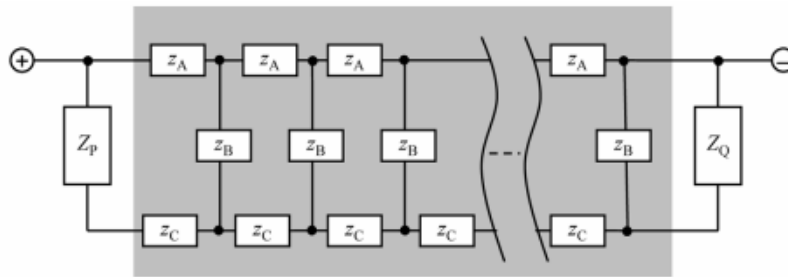
T-Type TLM arrangement
